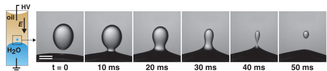
FIG. 1 (color). Left: diagram of the experimental apparatus. Right: time lapse images of a water droplet (1 mM KCl) undergoing electrically driven partial coalescence in 500 cSt PDMS oil. Field strength is 1.5 kV/cm; scale bar is 1 mm.
